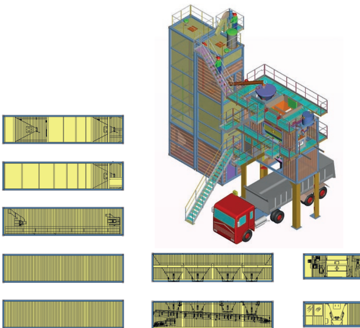
Containers configuration for a PHC-100 plant.
