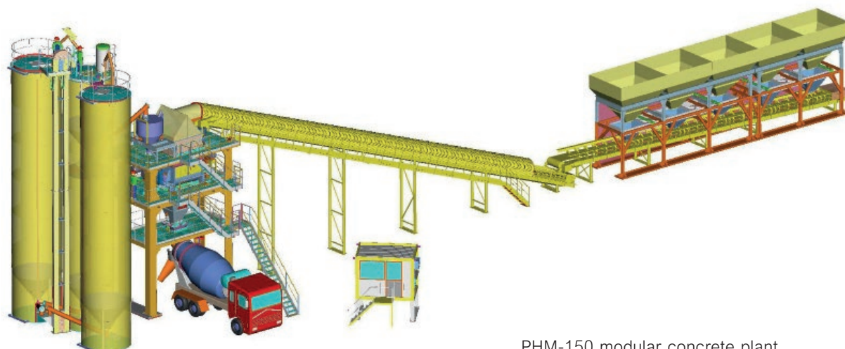
PHM-150 modular concrete plant.
